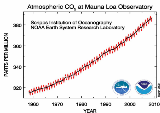
Figure 2. Recent changes in global atmospheric \text{CO}_2 concentrations.
